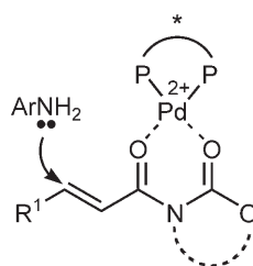
Figure 1. Chelation-assisted stereoselectivity.
