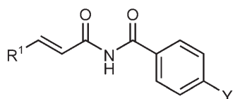
Figure 1. Chelation-assisted stereoselectivity.
