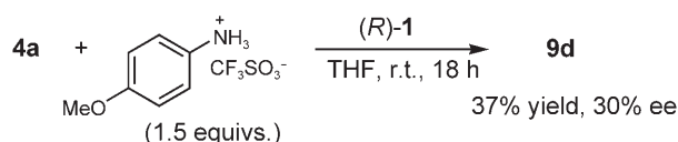
Scheme 5. Addition of trifluoromethanesulfonate salts.
