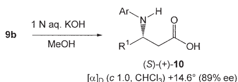
Scheme 4. Establishing the absolute configuration of 10 .
