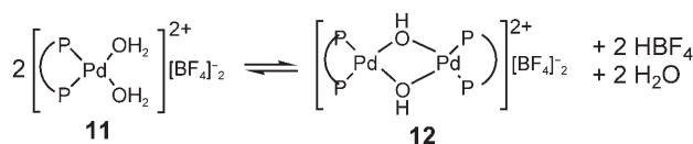
Scheme 6. Equilibrium mixture between monomeric and dimeric palladium(II) complexes.
