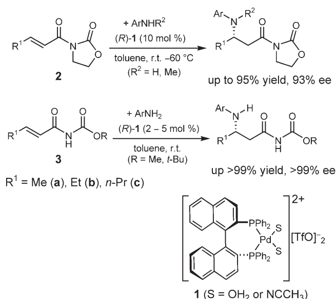
Scheme 1. Enantioselective addition of aromatic amines to \alpha,\beta -unsaturated N -oxazolidinones 2 and N -carbamates 3 catalysed by 1 .
