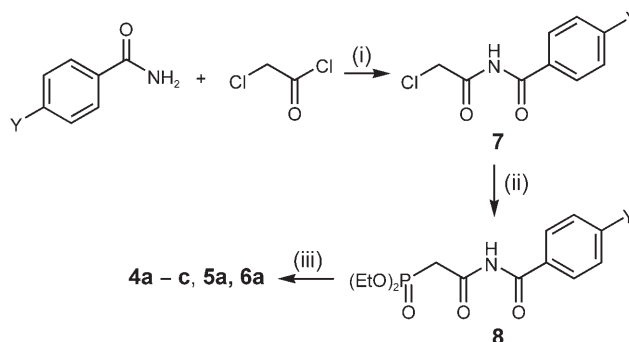
Scheme 2. Preparation of N -alkenyl N -imides 4a–c and 5a : (i) heat; (ii) P(OEt) 3 , heat; (iii) R 1 CHO, DBU, THF.
