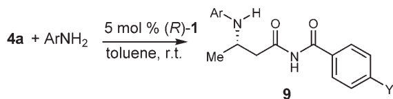
Scheme 3. Conjugate addition of aromatic amines to 4a .
